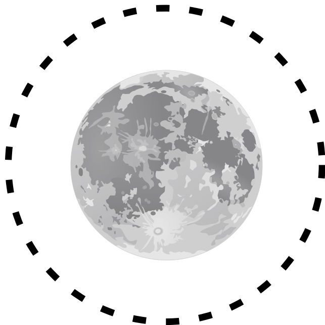
Orbit Around the Moon
