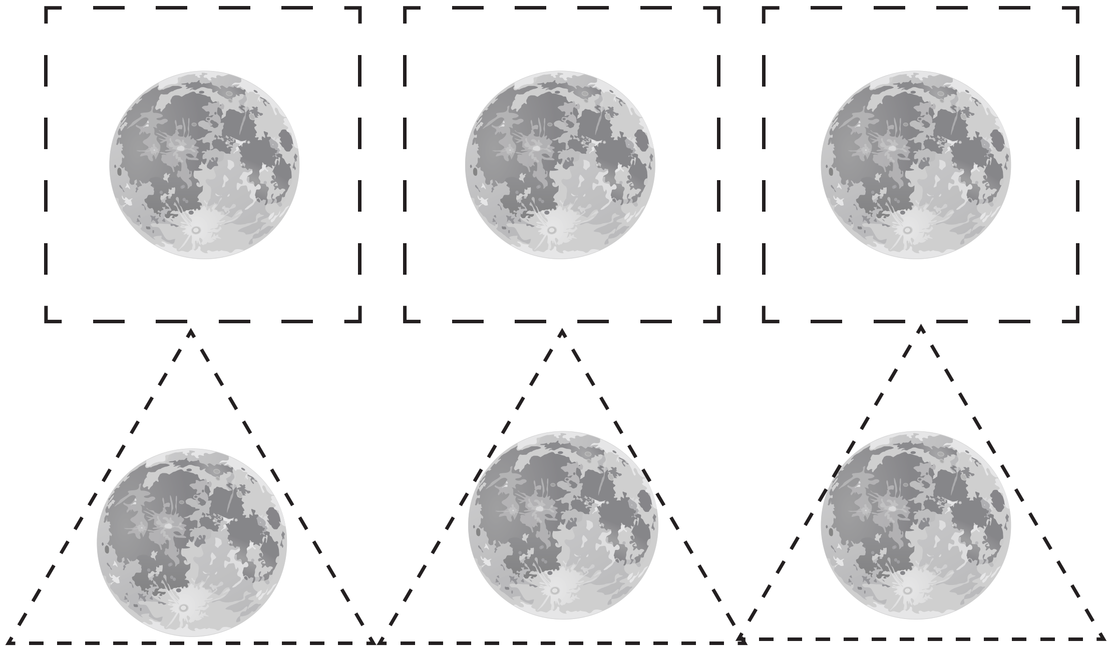
Orbit Around the Moon
